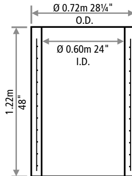
4 FT EXTENSION
