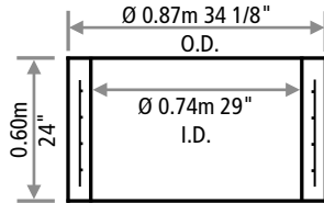
2 FT EXTENSION
