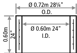
2 FT EXTENSION
