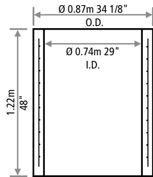
4 FT EXTENSION
