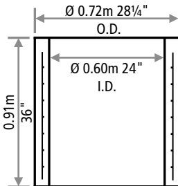
3 FT EXTENSION
