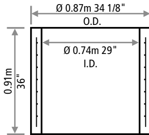
3 FT EXTENSION
