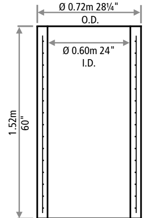
5 FT EXTENSION
