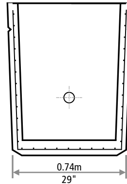
END VIEW
