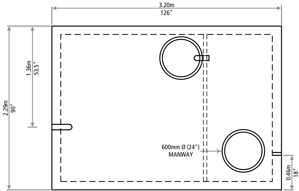
PLAN
