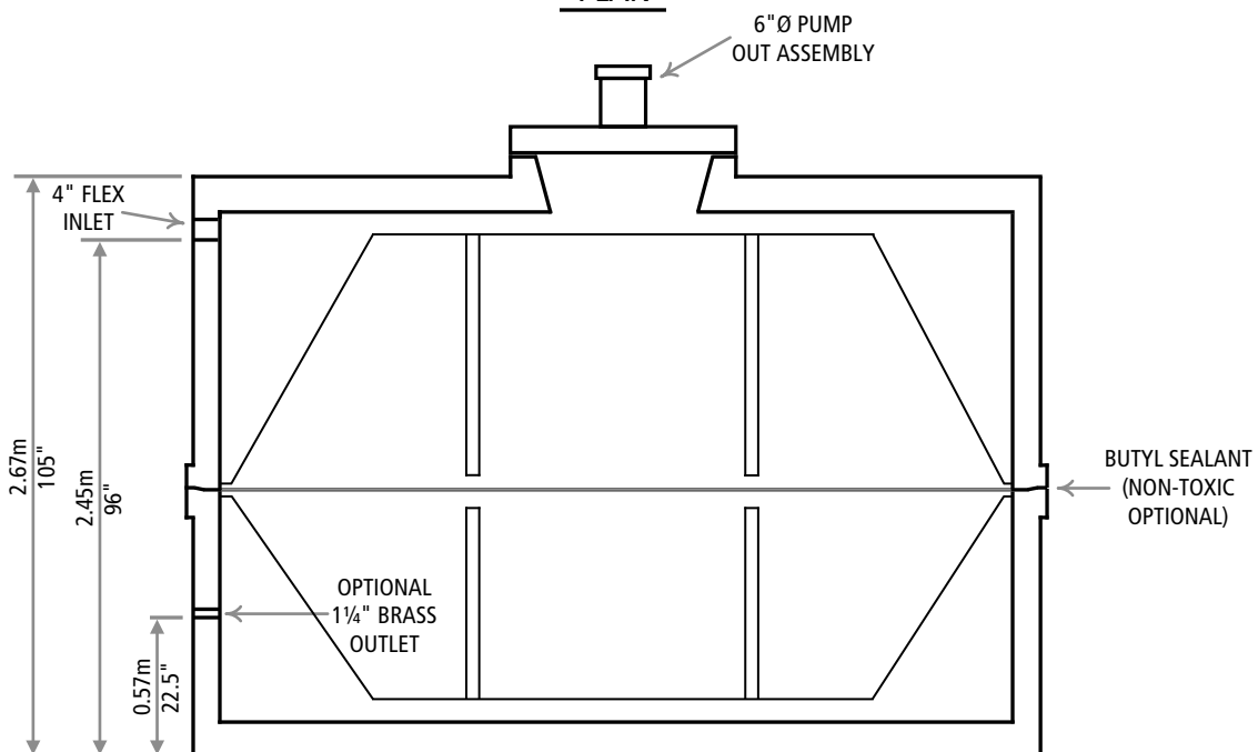
SECTION
