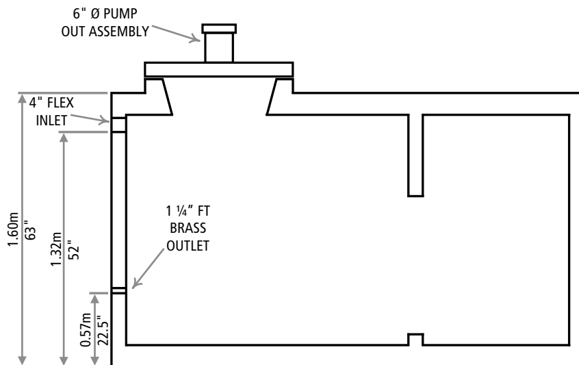
SECTION
