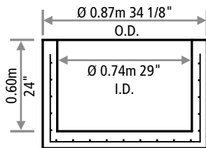
2 FT CATCH BASIN
