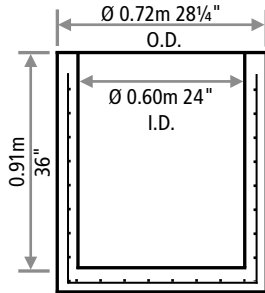
3 FT CATCH BASIN
