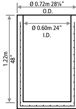
4 FT CATCH BASIN
