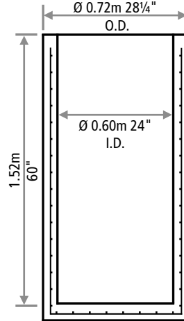
5 FT CATCH BASIN
