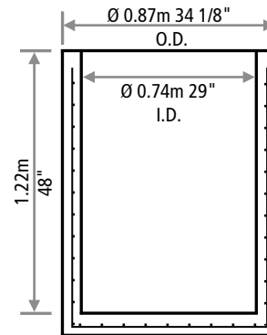
4 FT CATCH BASIN
