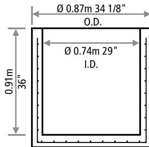
3 FT CATCH BASIN
