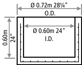
2 FT CATCH BASIN
